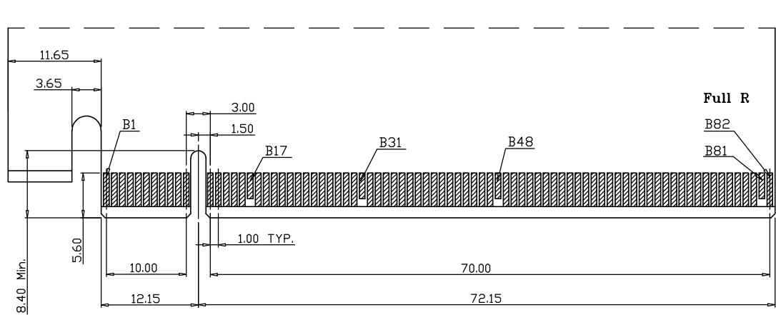
RECOMMENDED EDGE CARD PATTERN<PRIMARY SIDE>
